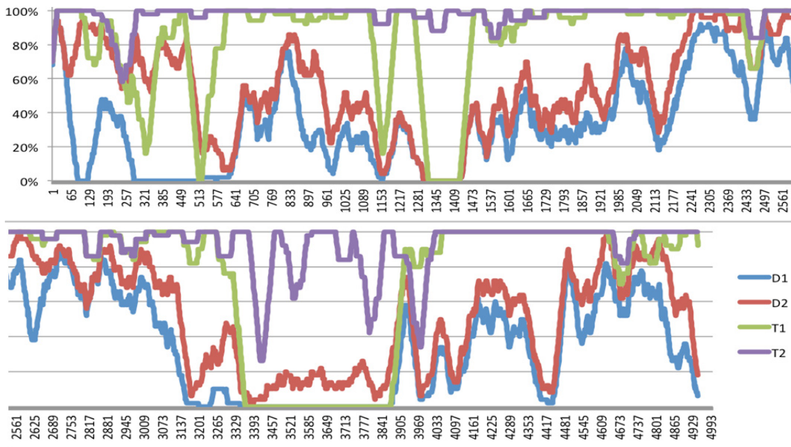
Figure 10: The success rate ( y -axis) versus time ( x -axis). Facial features are detected using the Viola–Jones-like detector without (D1) and with image compensation (D2). T1 and T2 show the success rate of the method proposed in (Wang, 2011) without and with image compensation, respectively. Note that this figure is warped.
